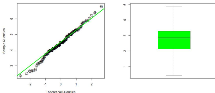
Figure 8: QQ-plot of the NEAPTW distribution and box plot for data 2.
