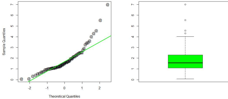
Figure 5: QQ-plot of the NEAPT distribution and box plot for data 1.
