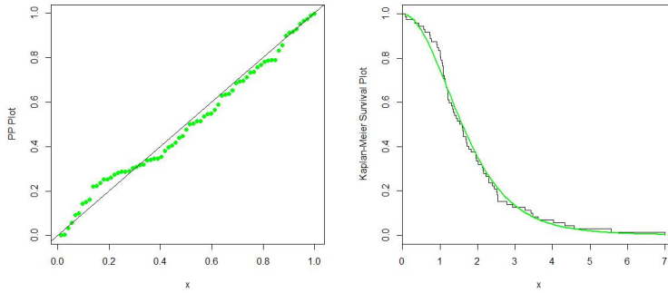
Figure 4: PP and Kaplan-Meier survival plots of the NEAPT distribution for data 1.
