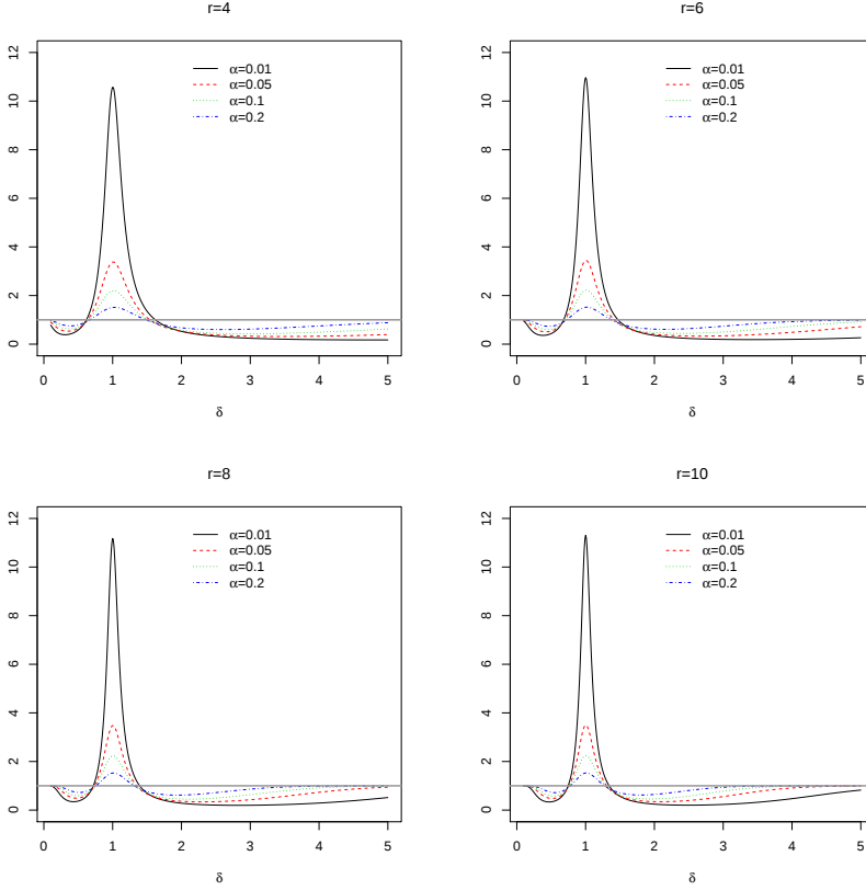
Figure 2: RE between the pretest and the risk-unbiased estimator for selected values of r = 4(2)10 and \alpha = 0.01, 0.05, 0.1, 0.2 with respect to \delta .
