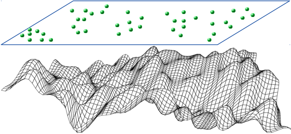
Figure 3: The hidden random field (surface) \Lambda_i(\mathbf{u}) controls the abundance and distribution of points of the Cox process X_i .
