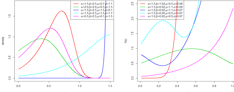
Figure 3: The pdf and hrf plots of OGLW-N distribution
