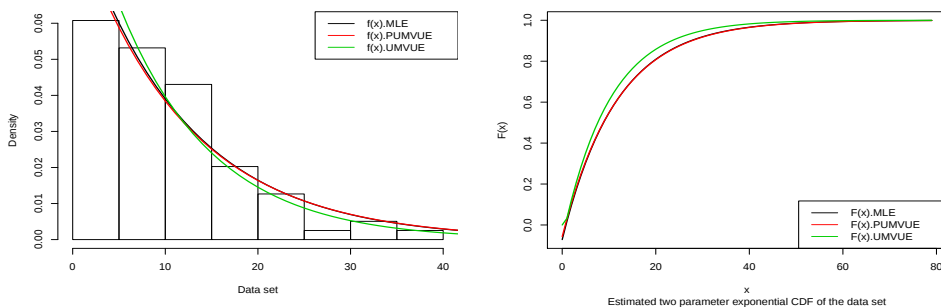
Figure 7: Graph of the estimated PDF and CDF of the two-parameter exponential distribution when the number of type-II censored sample is 75.
