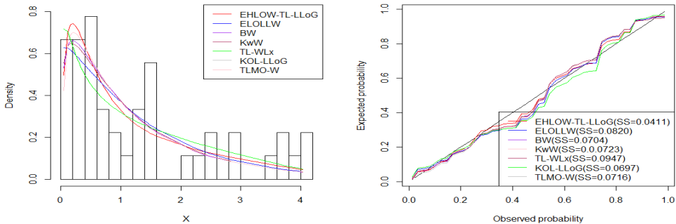
Figure 6: Fitted densities and probability plots for chemotherapy data
