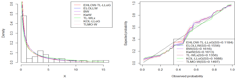
Figure 7: Fitted densities and probability plots for failure times data
