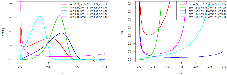
Figure 3: Plots of the pdf and hrf for the EHLOW-TL-U distribution
