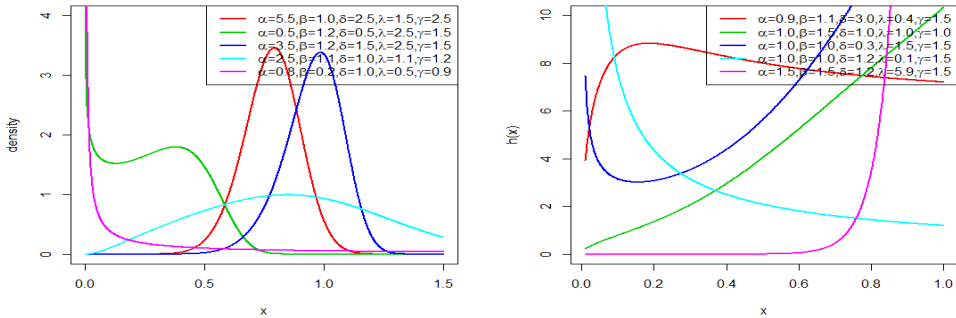
Figure 2: Plots of the pdf and hrf for the EHLOW-TL-BXII distribution
