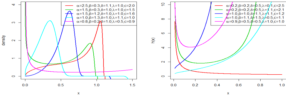
Figure 1: Plots of the pdf and hrf for the EHLOW-TL-P distribution
