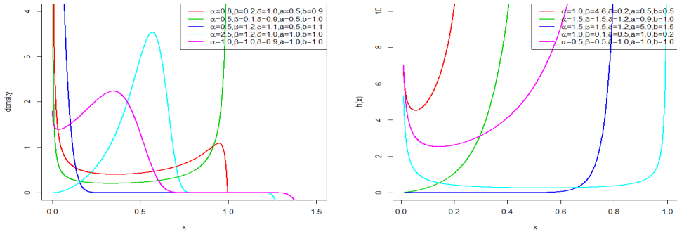
Figure 4: Plots of the pdf and hrf for the EHLOW-TL-Kw distribution
