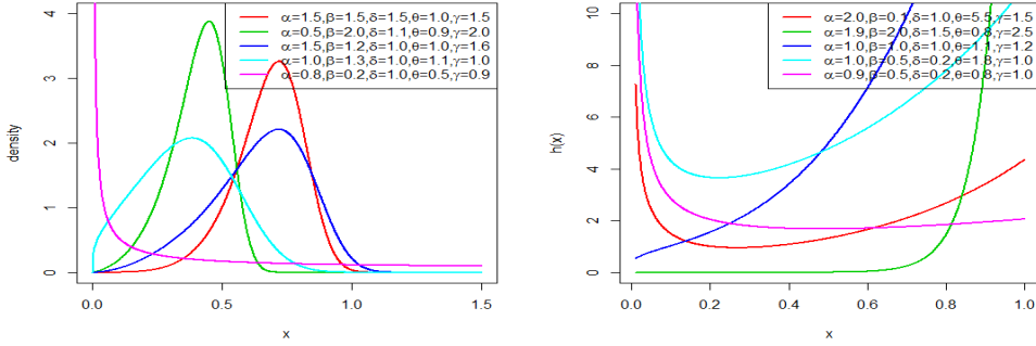
Figure 5: Plots of the pdf and hrf for the EHLOW-TL-W distribution
