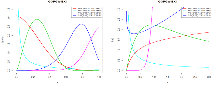
Figure 1: Plots of the pdf and hazard functions for the GOPGW-BXII Distribution.
