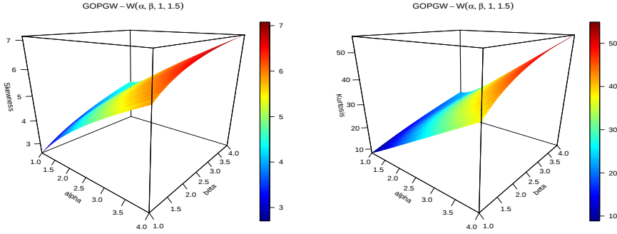
Figure 4: Skewness and kurtosis for the GOPGW-W distribution.
