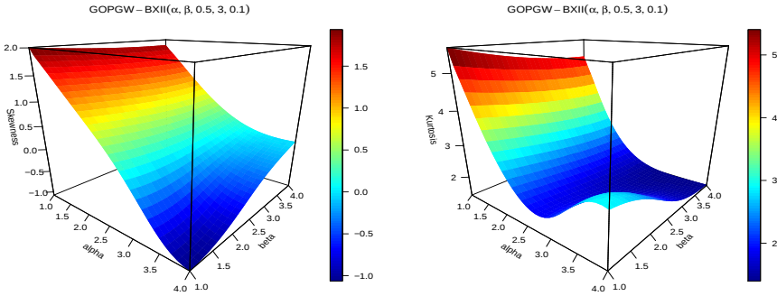
Figure 2: Skewness and kurtosis for the GOPGW-BXII distribution.
