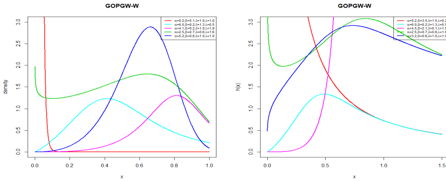
Figure 3: The density and hazard functions for the GOPGW-W distribution.
