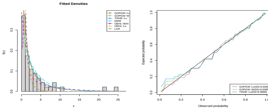
Figure 6: Fitted pdfs and cdfs plots of airborne communication transceiver data.
