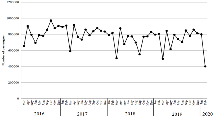
Figure 1: The number of passengers entered Tehran metro between 7 and 8am from March 2016 to March 2020.
