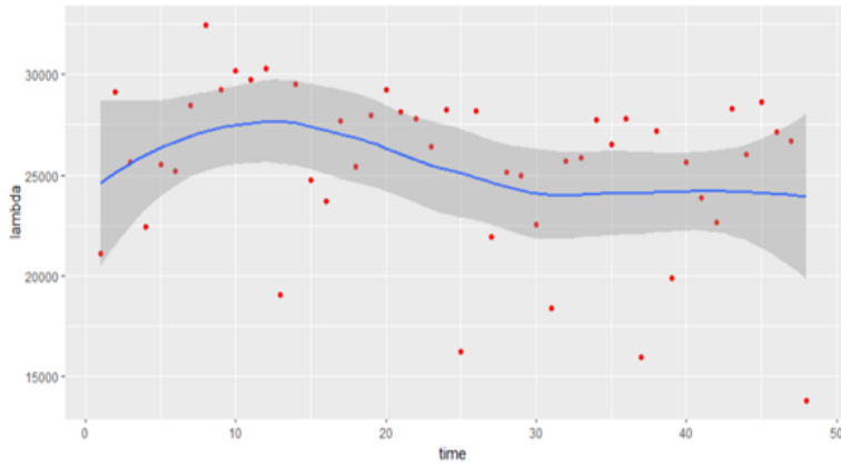
Figure 2: The intensity of the arrival of passengers from March 2016 to March 2020.
