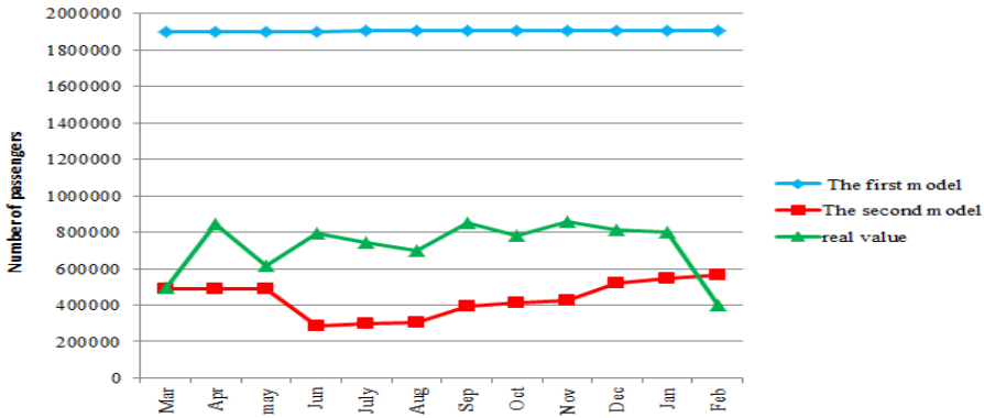
Figure 3: Comparison of the mean prediction of the number of incoming passengers in the two models presented with the actual value
